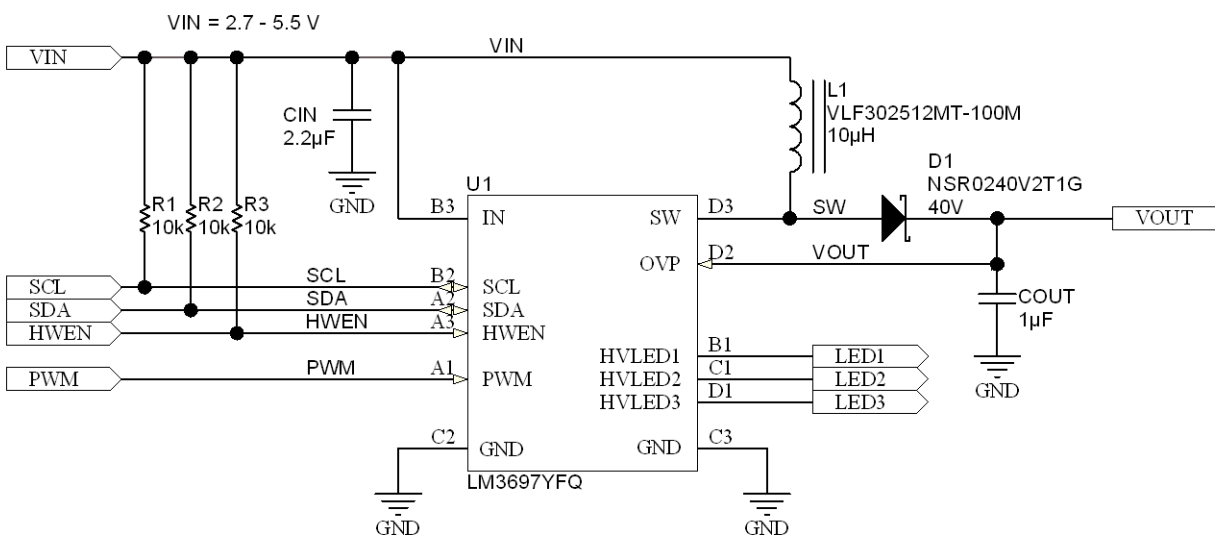
Figure 13. LM3697 Schematic
