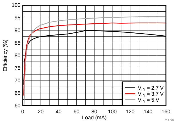
图 153. LCM Boost Efficiency
