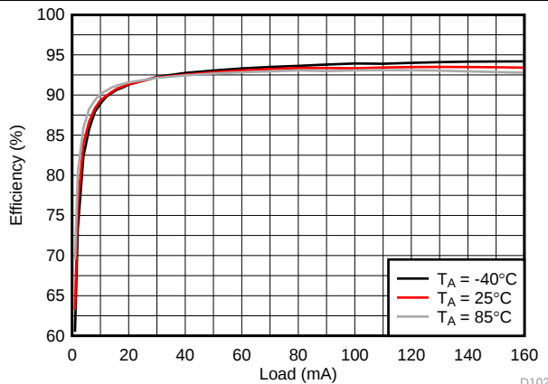
图 152. LCM Boost Efficiency
