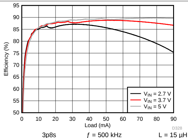
图 140. Backlight System Efficiency
