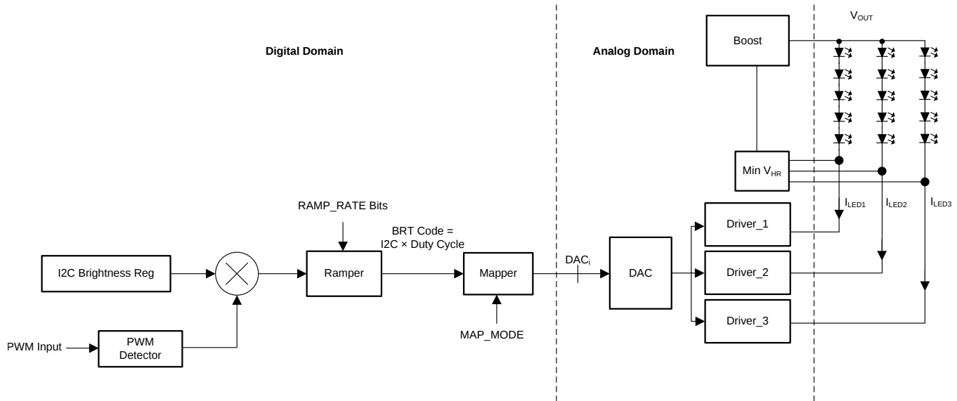
图 36. ( I^2C + PWM) Brightness Control, PWM Ramper Enabled
