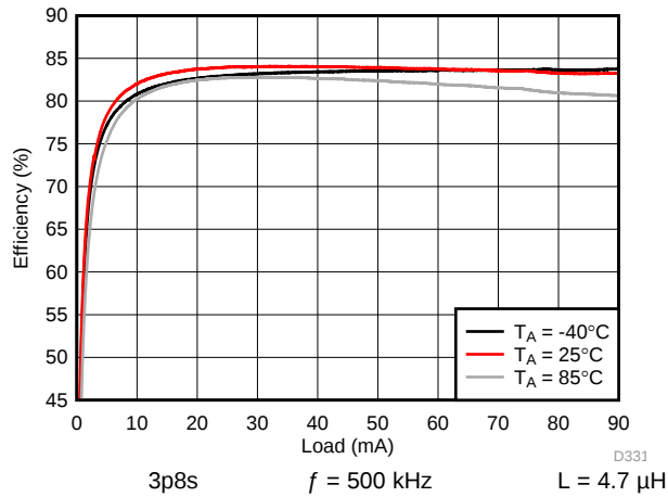
图 145. Backlight Boost Efficiency
