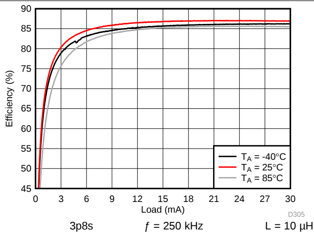
图 117. Backlight Boost Efficiency
