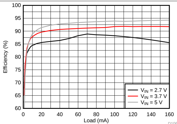
图 154. LCM Boost Efficiency
