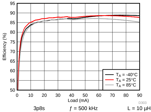
图 115. Backlight Boost Efficiency
