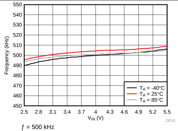
图 11. Backlight Boost Frequency
