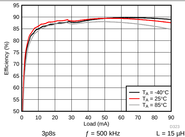
图 135. Backlight Boost Efficiency
