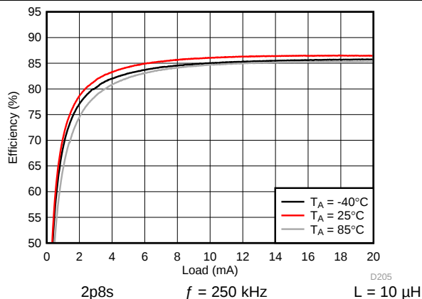
图 73. Backlight Boost Efficiency
