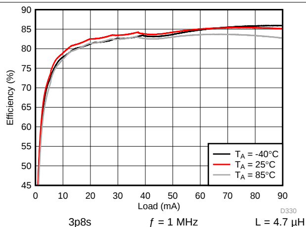
图 142. Backlight System Efficiency
