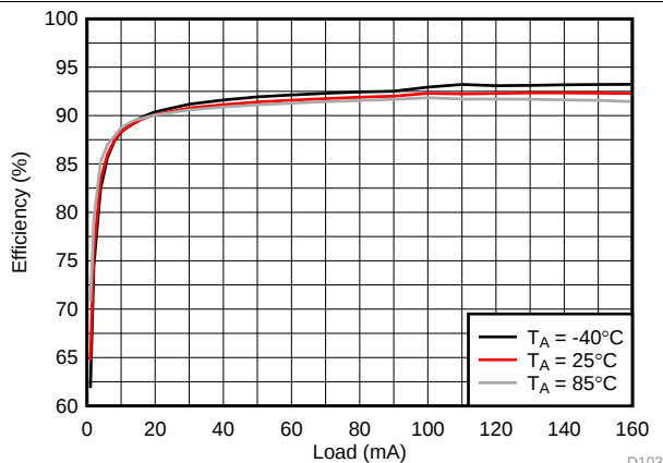
图 151. LCM Boost Efficiency
