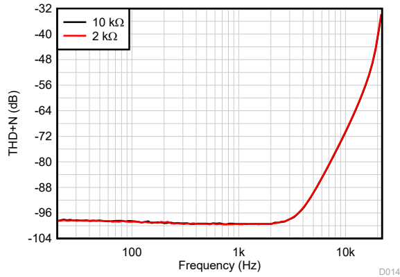
G = -1 , f = 1\text{kHz} , \text{BW} = 80\text{kHz} , V_{\text{OUT}} = 10\text{V}_{\text{PP}} , R_L 连接到 V^- 请参阅图 7-3
