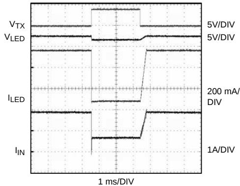
Figure 32. Tx-Mask Event
