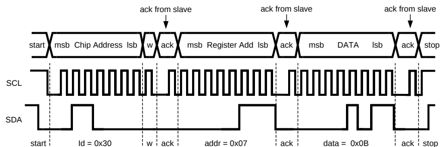
Figure 50. Write Cycle
