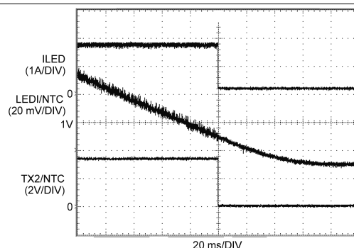
Figure 20. NTC-Mode Operation
