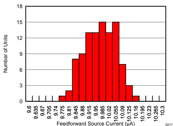
Figure 16. Feedforward Source Current ( I_{\text{FF}} ) Variation ( I_{\text{VAC}}=100\text{ }\mu\text{A} , Temperature = 25^{\circ}\text{C} )
