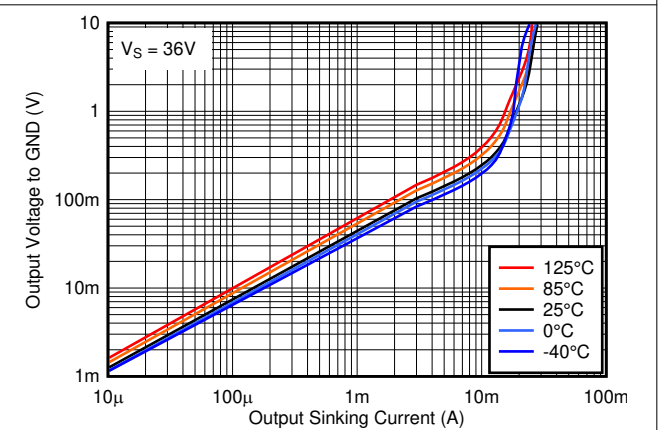
图 6-22. Output Low Voltage vs. Output Sinking Current at 36V
