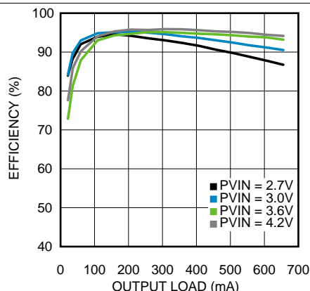
Figure 6. PFM Efficiency
