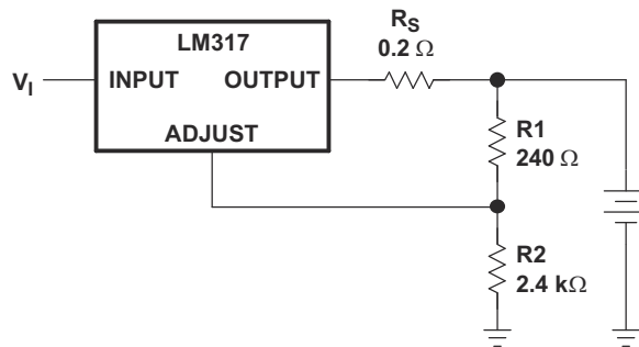
图 8-11. Battery-Charger Circuit
