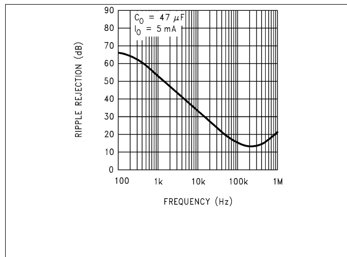
Figure 15. LM2990-12 and LM2990-15 Ripple Rejection
