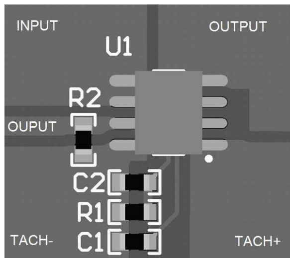
Figure 48. Layout Recommendation
