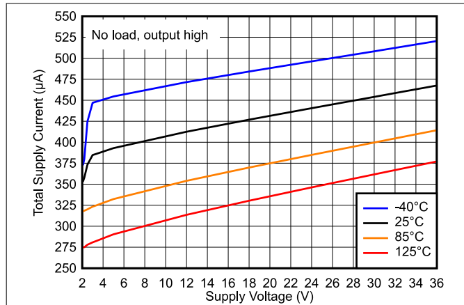
图 2-1. Total Supply Current vs. Supply Voltage
