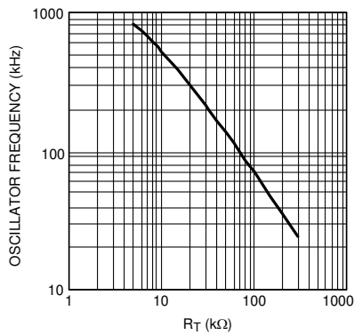
图 5-1. Oscillator Frequency vs R_T
