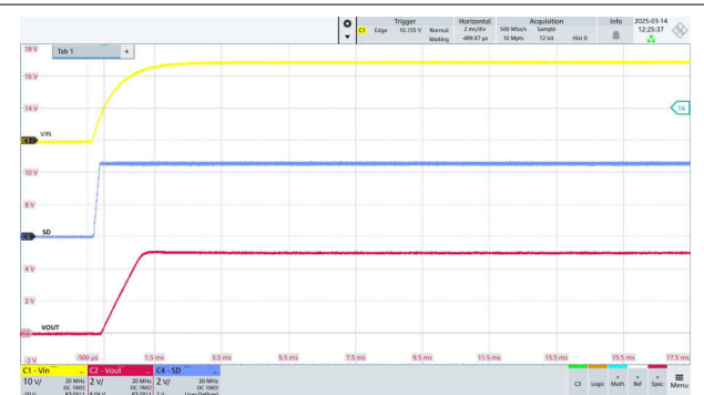
图 7-11. Start-Up Operation
