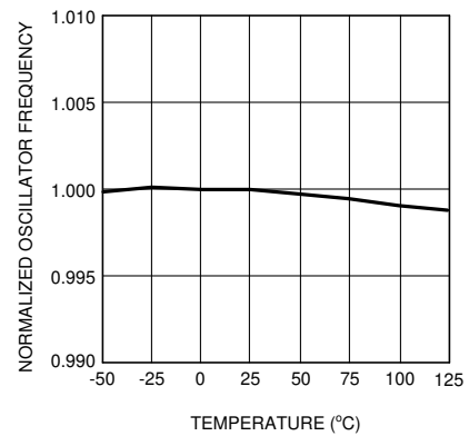
图 5-2. Oscillator Frequency vs Temperature
