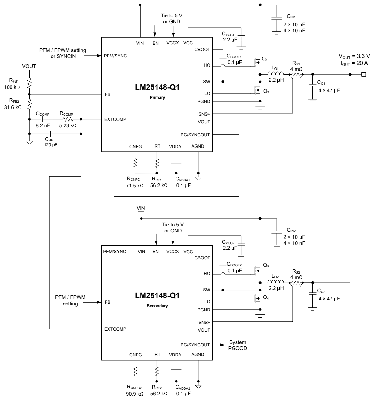
图 9-28. Application Circuit 3 with Two LM25148-Q1 Buck Regulators Switching at 400 kHz
