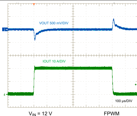
图 9-34. Load Transient, 0 A to 20 A
