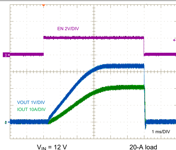
图 9-32. ENABLE ON and OFF Characteristic
