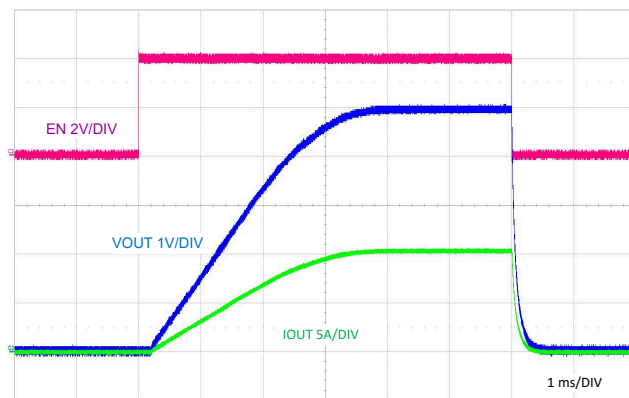
图 9-25. ENABLE ON and OFF Characteristic
