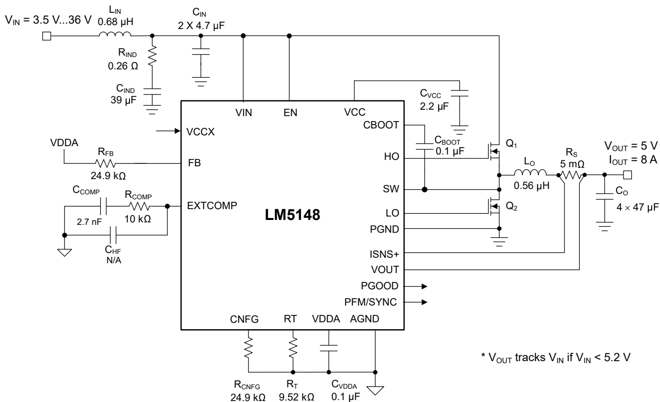
图 9-4. Application Circuit 1 With LM25148-Q1 Buck Regulator Switching at 2.1 MHz
