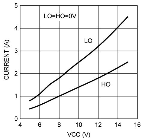
图 5-2. Driver Source Current vs VCC
