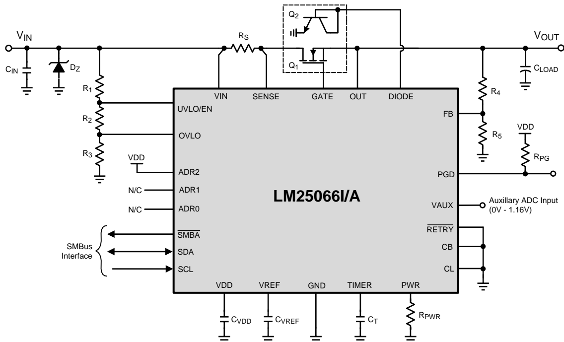
Figure 31. Typical Application Circuit
