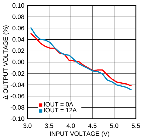
Figure 5. Line Regulation
