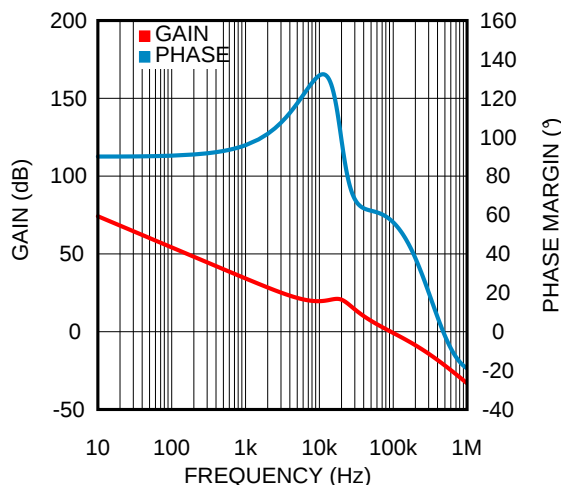
Figure 35. Loop Response
