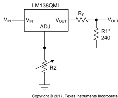
图 16. Regulator With Line Resistance in Output Lead
