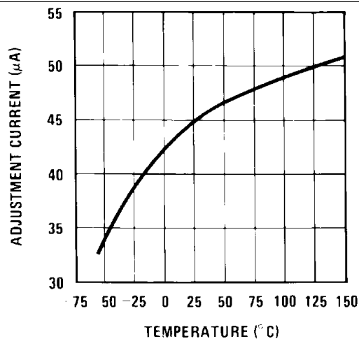
图 6. Adjustment Current
