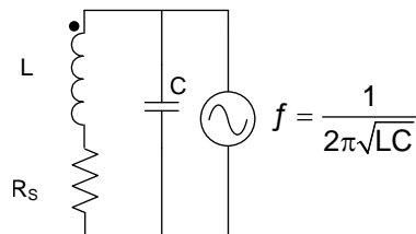
Figure 47. LC Tank
