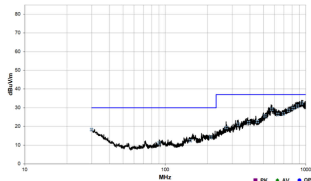
图 10-3. ISOW7741 Radiated Emissions versus CISPR32B line (Blue)
