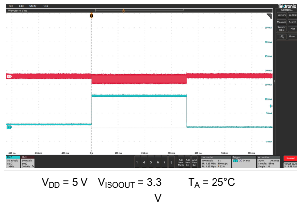
图 7-25. 10-mA to 110-mA Load Transient Response
