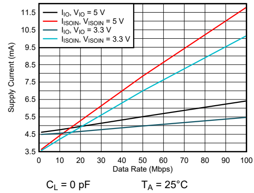
图 7-12. ISOW7740 Channel Supply Currents vs Data Rate For C_L = 0\text{ pF}
