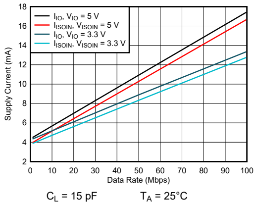
图 7-15. ISOW7742 Channel Supply Currents vs Data Rate For C_L = 15 \text{ pF}
