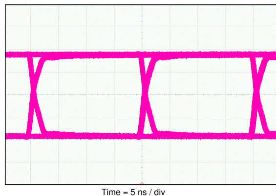
图 9-6. Eye Diagram at 50 Mbps PRBS 2^{16} - 1 , 1.8 V and 25°C
