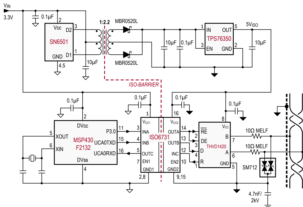
图 9-1. Isolated RS-485 Interface Circuit
