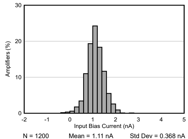
图 7-6. Typical Distribution of Noninverting Input Bias Current
