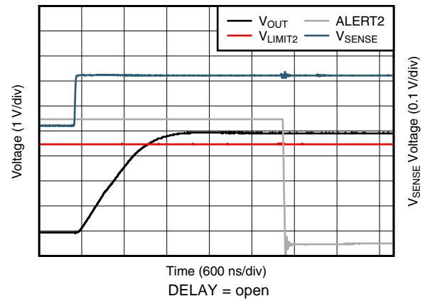
图 32. Comparator 2 Total Propagation Delay (INA303)
