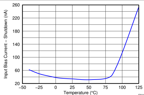
图 7-14. Input Bias Current vs. Temperature, Shutdown
