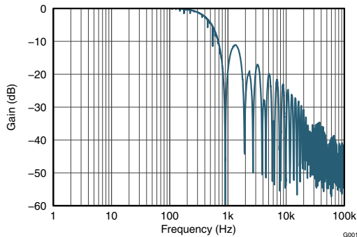
图 7-1. Frequency Response
