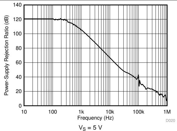
图 10. Power-Supply Rejection Ratio vs Frequency
