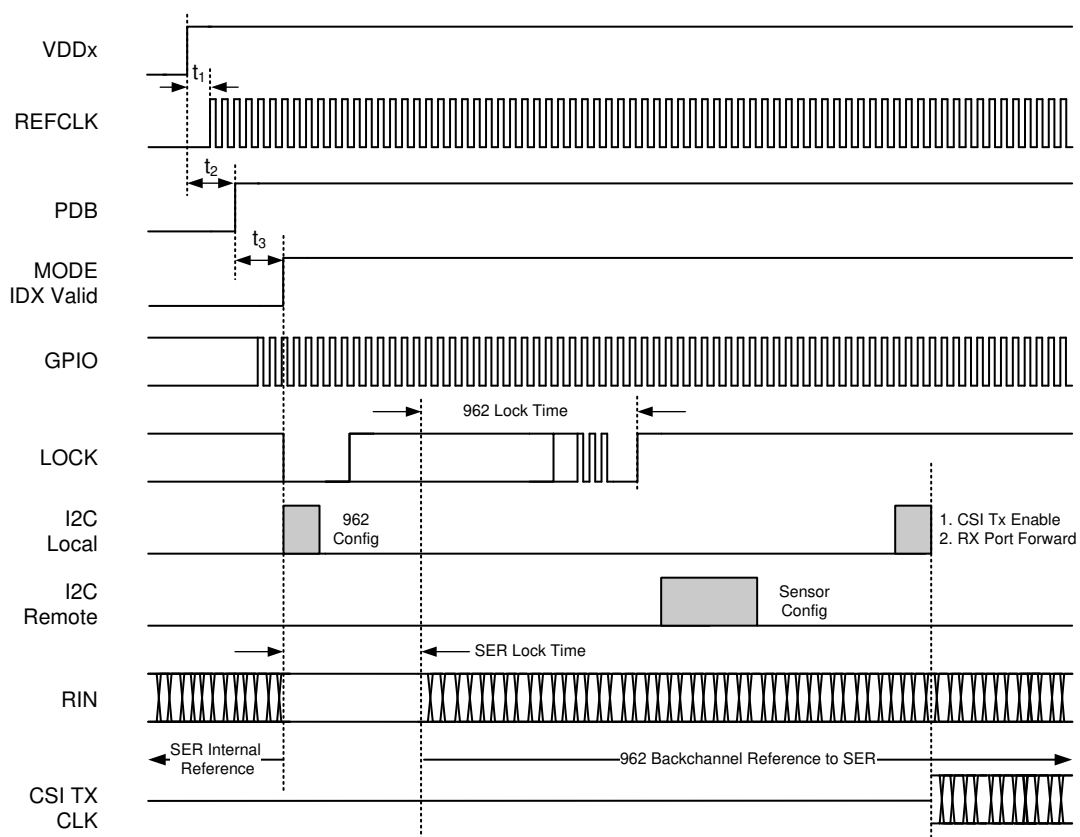
图 8-15. Power-Up Sequencing With Synchronous Clocking Mode
