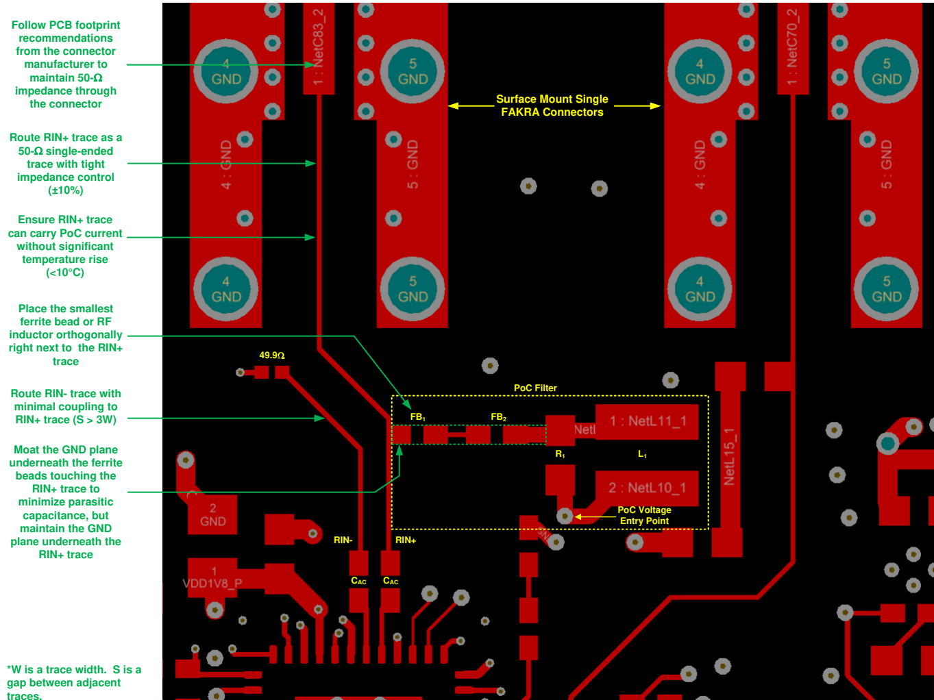
图 8-18. Example Routing of FPD-Link III Traces to a Single Mini-Fakra Connector and PoC Components
