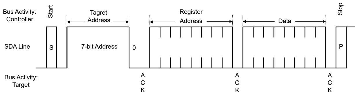
图 7-16. Serial Control Bus — WRITE
