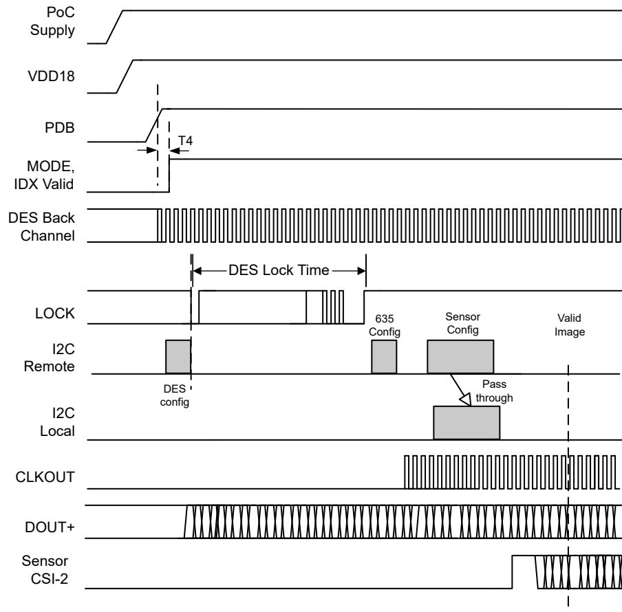
图 9-2. Initialization Sequence: Synchronous Clocking Mode
