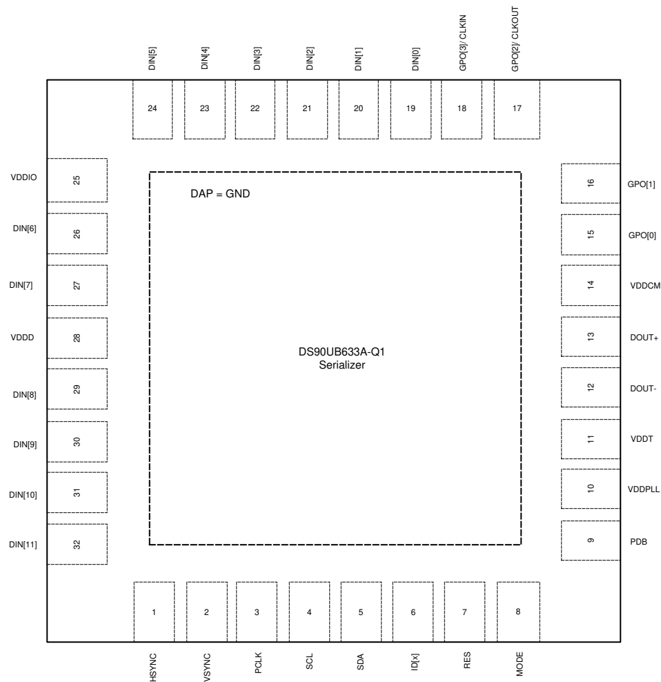
图 5-1. RTV Package 32-Pin WQFN Top View
