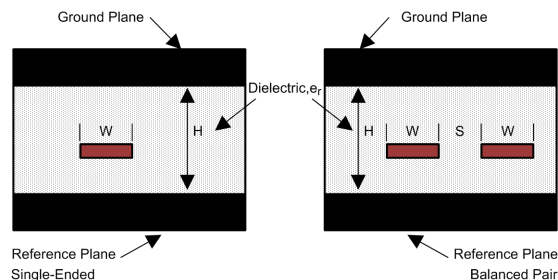
Figure 17. Stripline Topology
