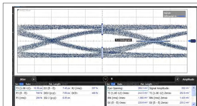
图 6-3. Through Baseline Calibration Trace Setup
