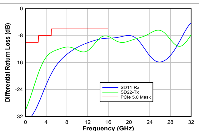
图 6-2. Typical Differential Return Loss
