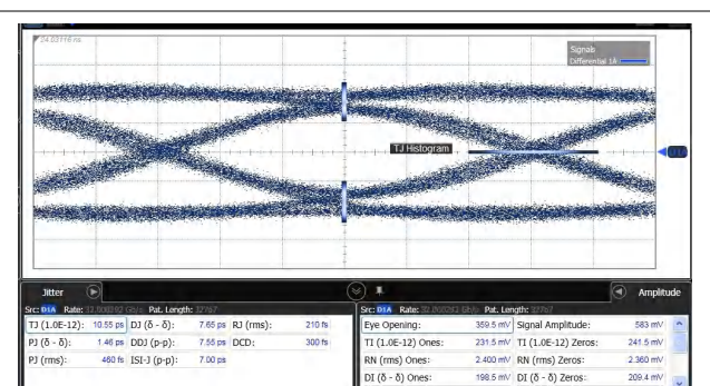
图 6-4. Through the DS320PR1601 with DUT EQ = 0
