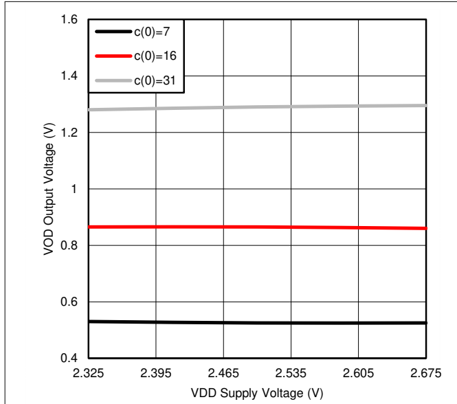
图 5-1. Typical VOD versus Supply Voltage
