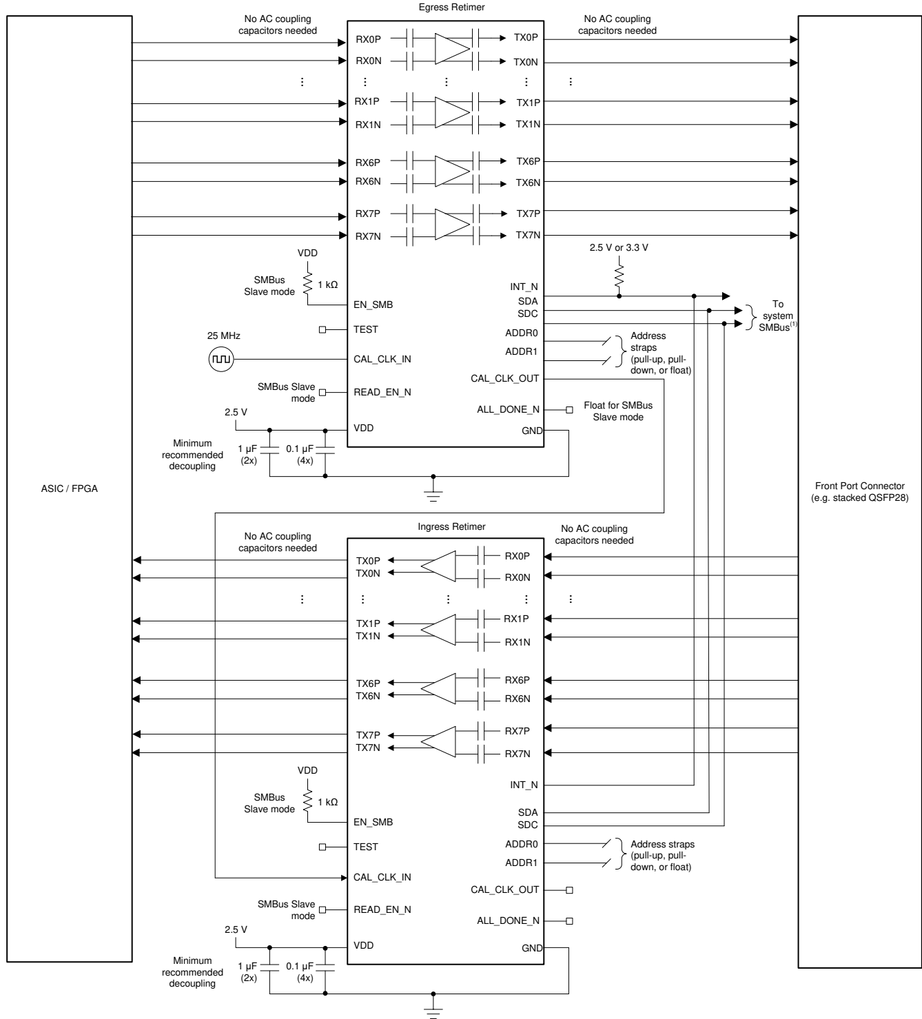
图 7-5. Front-Port Application Schematic
