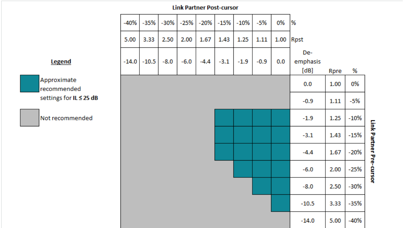
图 6-8. Guideline for Link partner FIR Settings When IL \leq 25 dB
