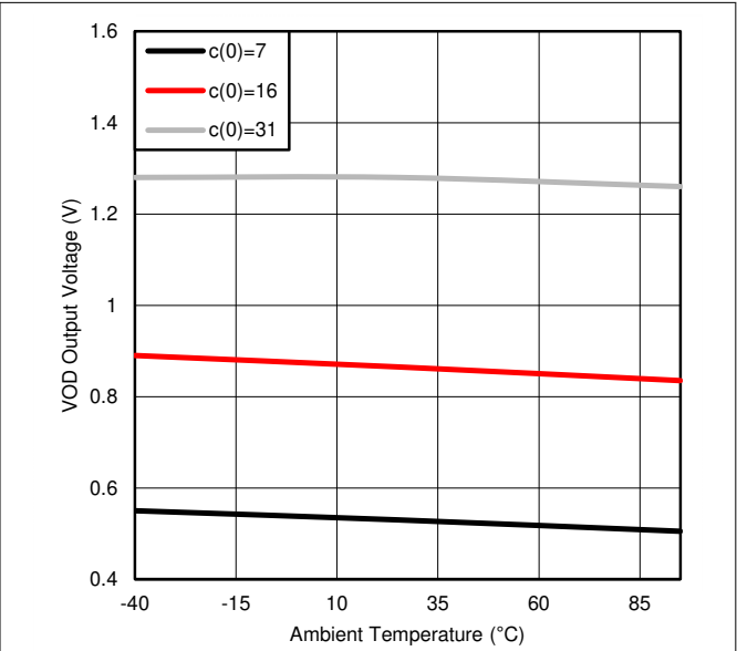
图 5-2. Typical VOD versus Temperature
