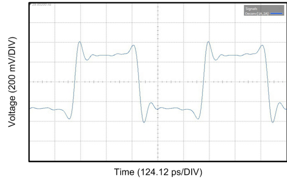
图 19. DS250DF810 FIR Transmit Equalization while Operating at 25.78125 Gbps
