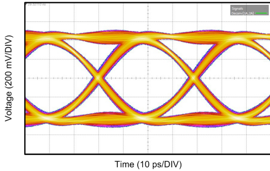
图 18. DS250DF810 Operating at 25.78125 Gbps
