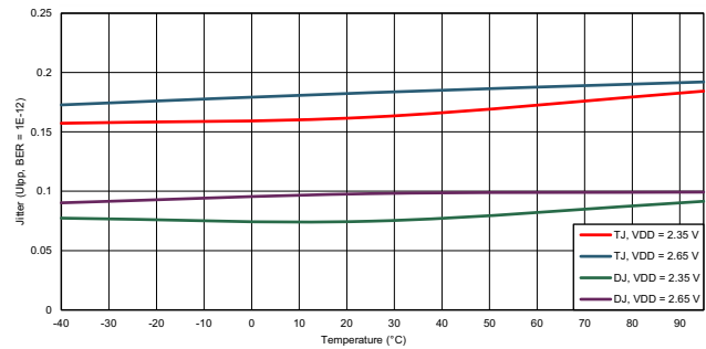
图 4. Typical Output Jitter versus Temperature at 25.78125Gbps
