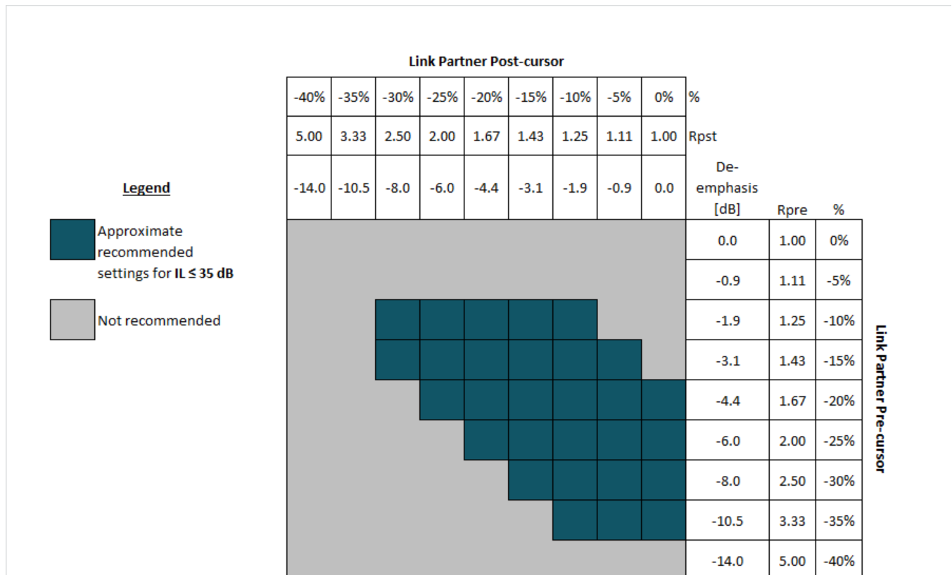
图 13. Guideline for Link Partner FIR Settings When IL \leq 35 dB
