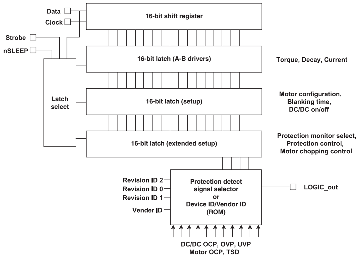
Figure 6. Serial Interface A-B
