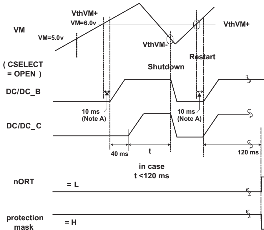
Figure 22. Power Down (Glitch on V_M )
