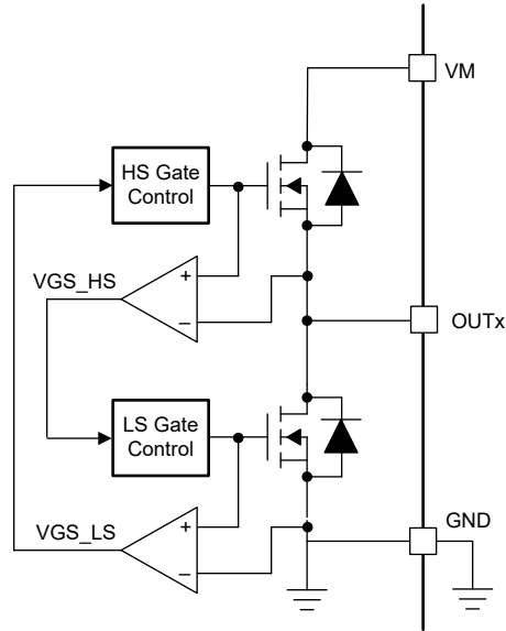
图 8-18. Cross Conduction Protection
