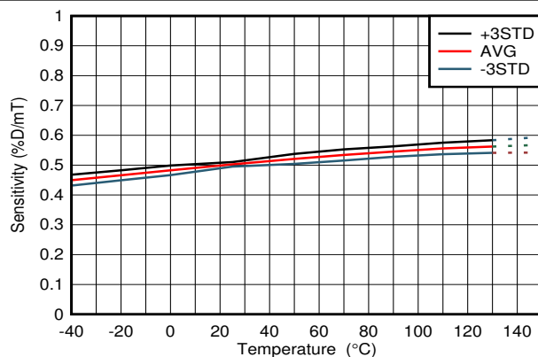
图 6-13. Sensitivity vs Temperature
