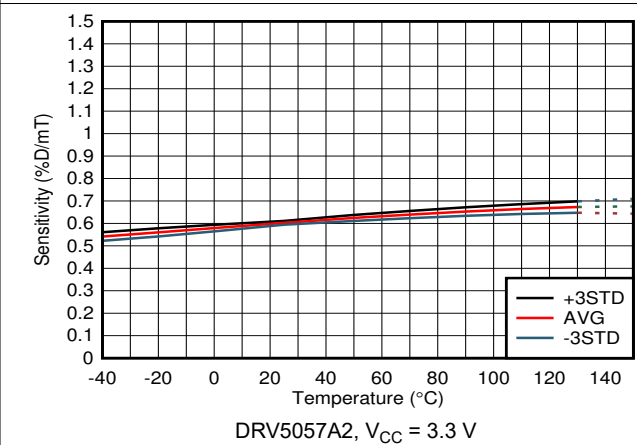
图 6-12. Sensitivity vs Temperature
