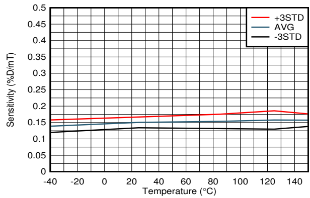
图 6-20. Sensitivity vs Temperature
