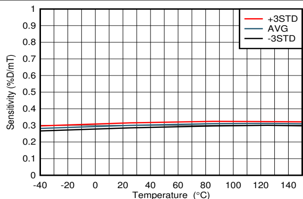
图 6-16. Sensitivity vs Temperature
