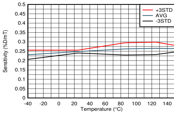
图 6-19. Sensitivity vs Temperature
