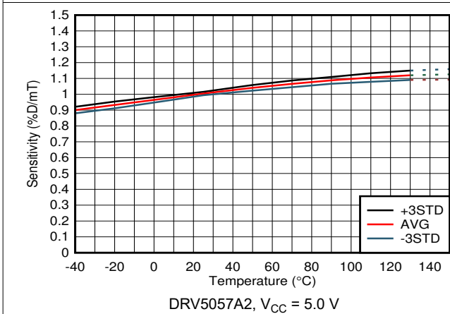
图 6-11. Sensitivity vs Temperature
