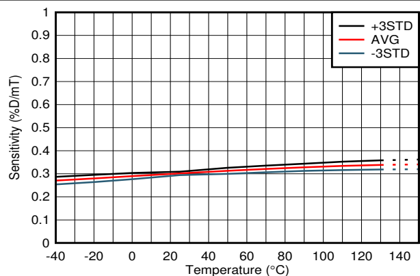
图 6-14. Sensitivity vs Temperature
