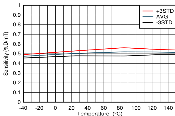
图 6-15. Sensitivity vs Temperature
