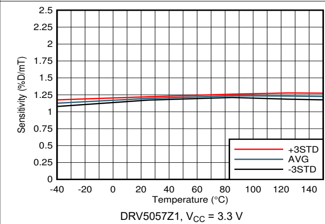
图 6-10. Sensitivity vs Temperature
