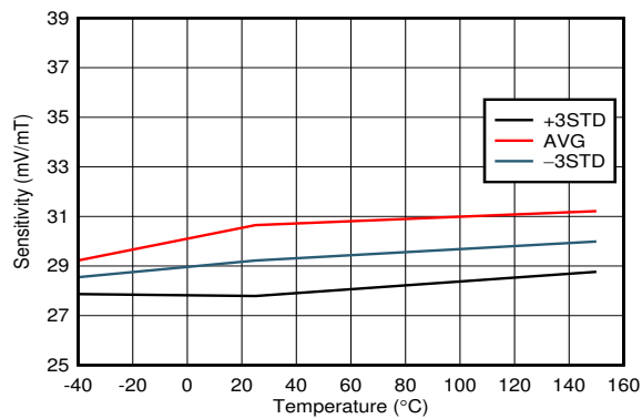
DRV5056Z3, V CC = 3.3V
