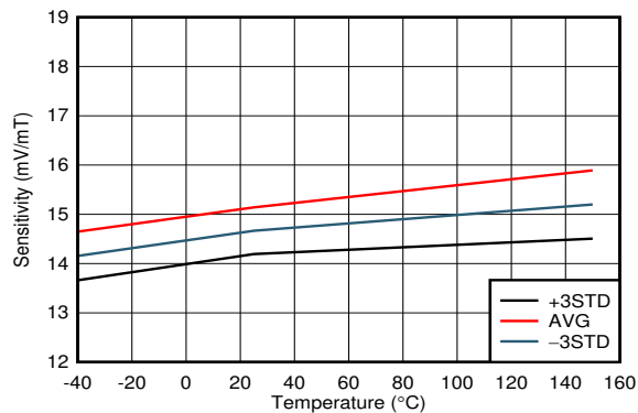
DRV5056Z4, V CC = 3.3V
