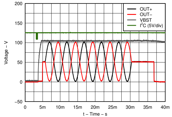
图 6-10. Typical Waveform
