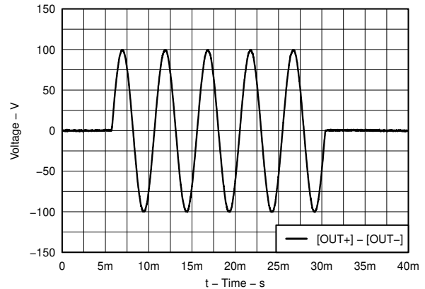
图 6-12. Typical Waveform - Differential
