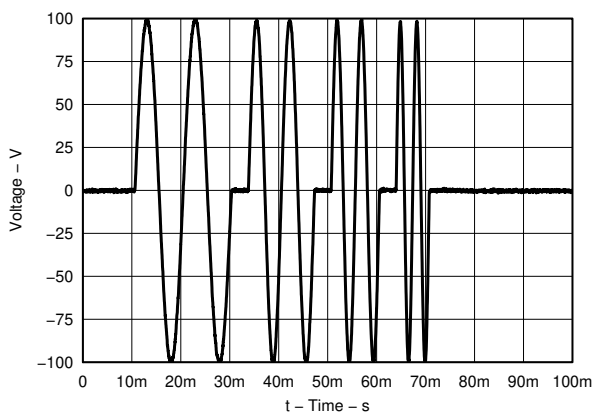
图 6-18. Example Waveform - Frequency
