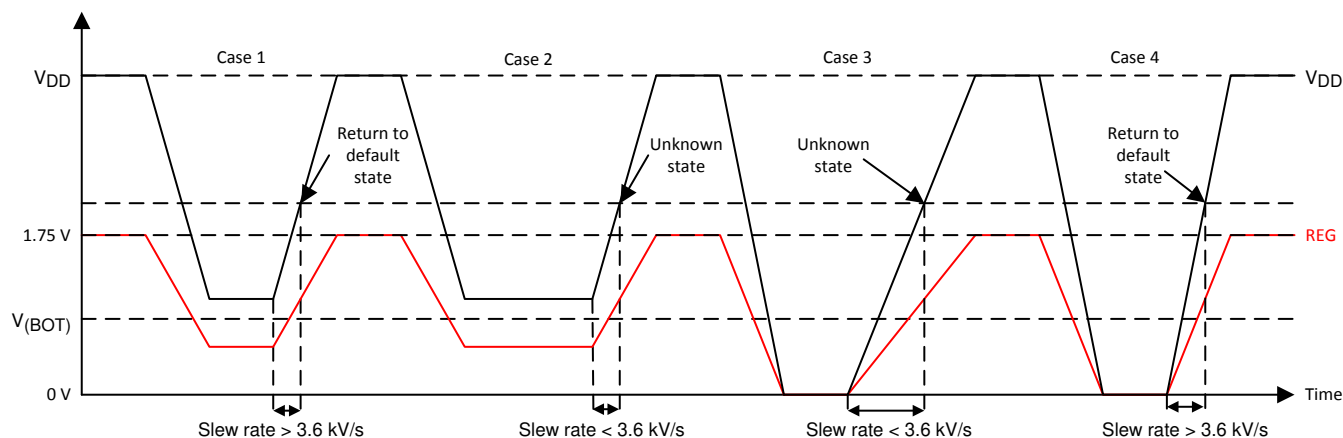
图 7-2. Brownout Behavior
