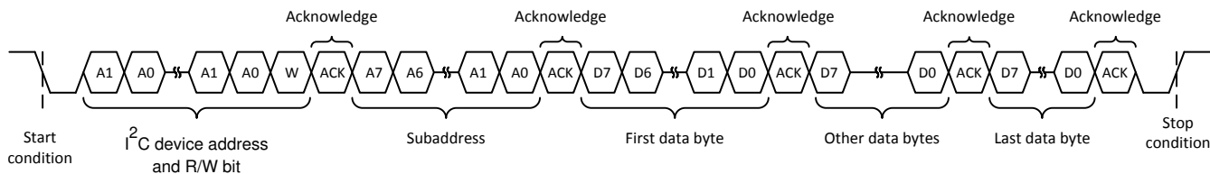
图 7-12. Multiple-Byte Write Transfer
