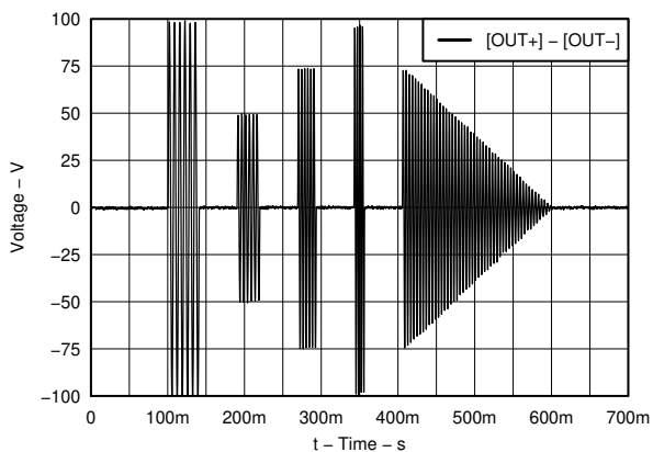
图 6-20. Example Waveform - Pinball Effect
