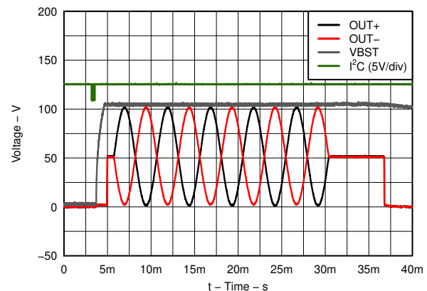
图 8-4. Typical Waveform
