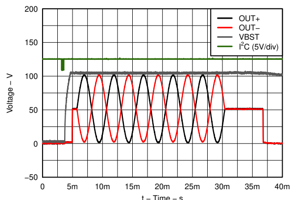
图 8-4. Typical Waveform
