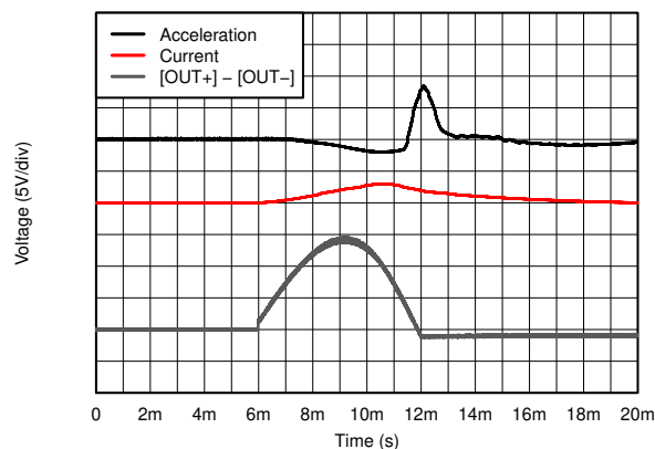
图 8-5. Voltage and Acceleration vs Time (1/2 Sine Wave)
