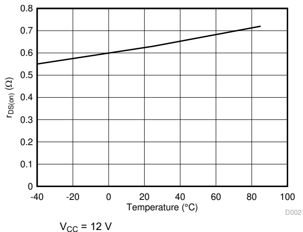
图 6-2. r DS(on) vs Temperature When V CC = 12 V
