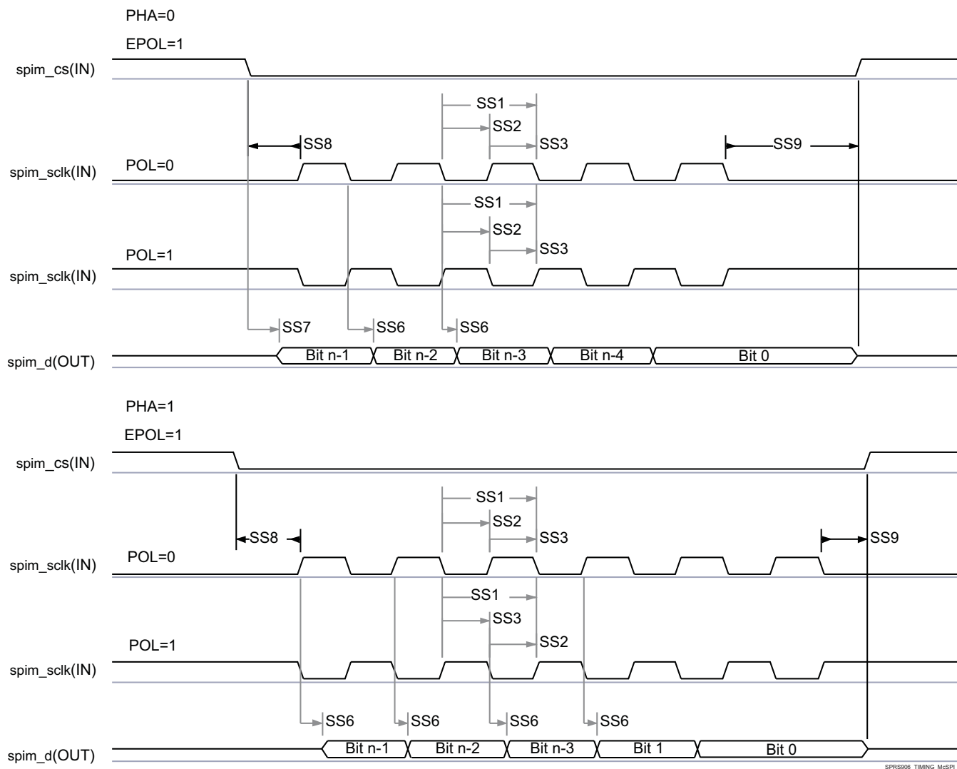
图 7-35. McSPI - Slave Mode Transmit
