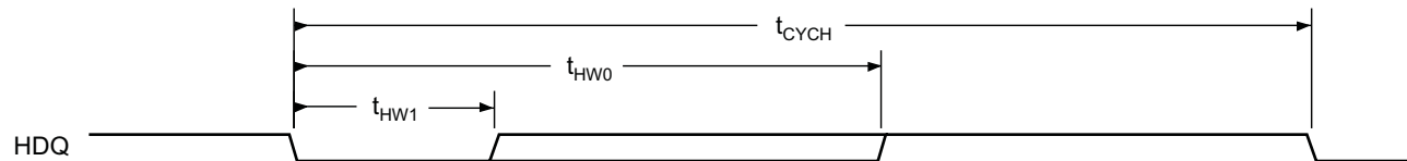
图 7-26. Device HDQ Interface Bit Read Timing (Data)
