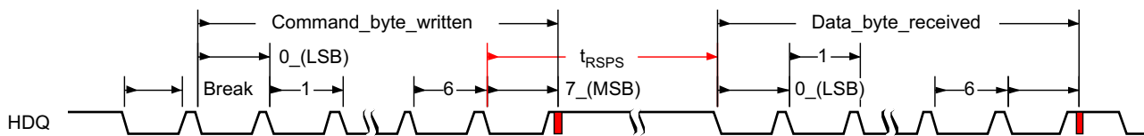
图 5-44. HDQ Communication Timing
