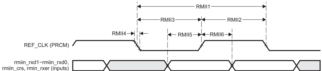
图 5-73. GMAC Receive Interface Timing RMIIn operation
