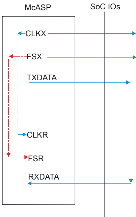
图 5-63. McASP1-8 CO-FO- – SYNC Mode
