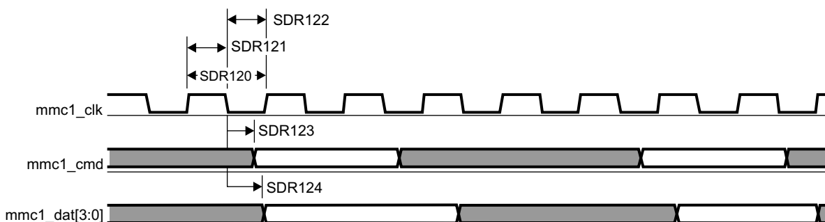
图 5-83. MMC/SD/SDIO in - High Speed SDR12 - Transmitter Mode
