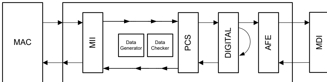
图 8-6. Digital loopback without data generator
