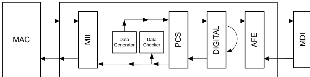
图 8-5. Digital loopback with data generator
