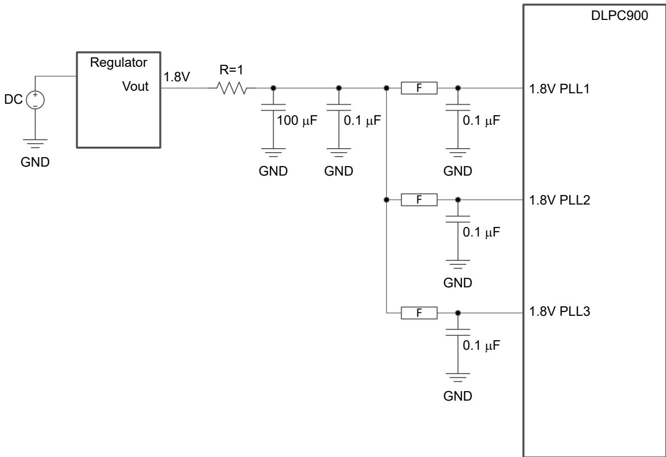
图 9-2. Recommended Filter Topology for PLL 1.8-V Supplies
