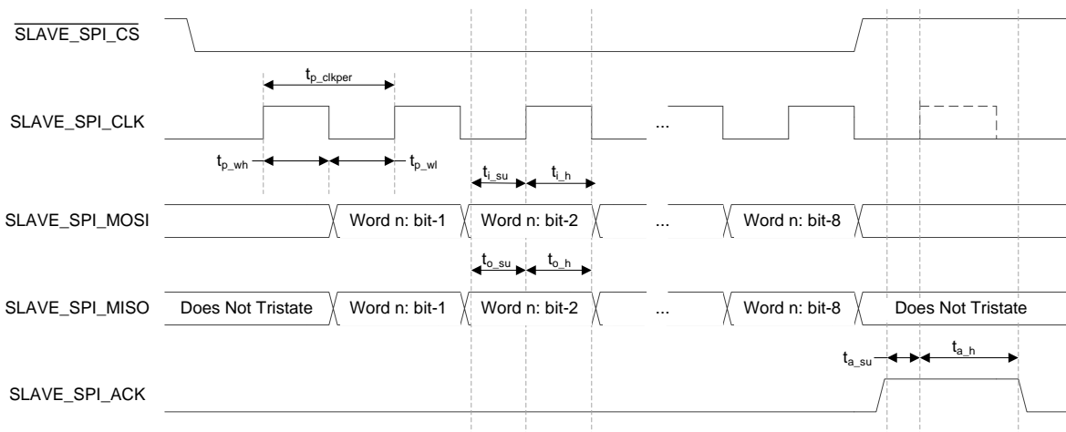
Figure 5. SPI Timing
