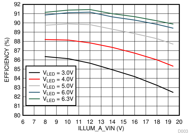
图 8-14. Illumination Driver Plus Power FETS Efficiency vs V_{ILLUM\_A\_IN}
