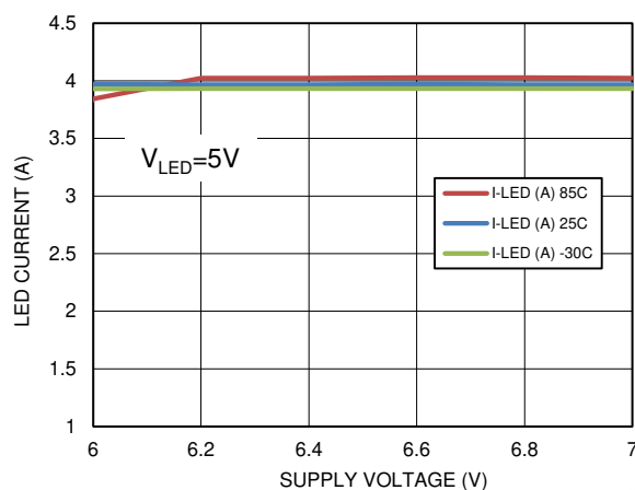
图 8-11. 4-A Led Current at V_{LED} = 5\text{ V}
