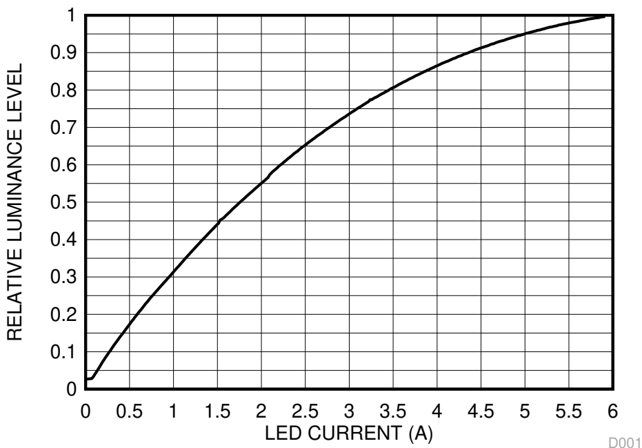
图 9-2. Luminance vs LED Current
