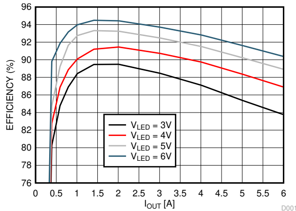
图 8-13. Illumination Driver Plus Power FETS Efficiency ( V_{ILLUM\_A\_IN} = 12\text{ V} )
