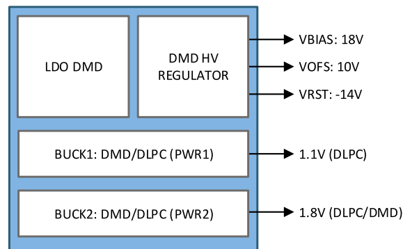
图 8-15. DMD Supplies Blocks
