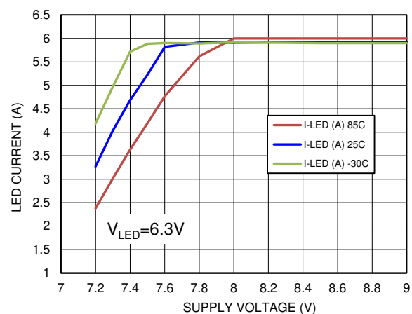
图 8-12. 6-A Led Current at V_{LED} = 6.3\text{ V}
