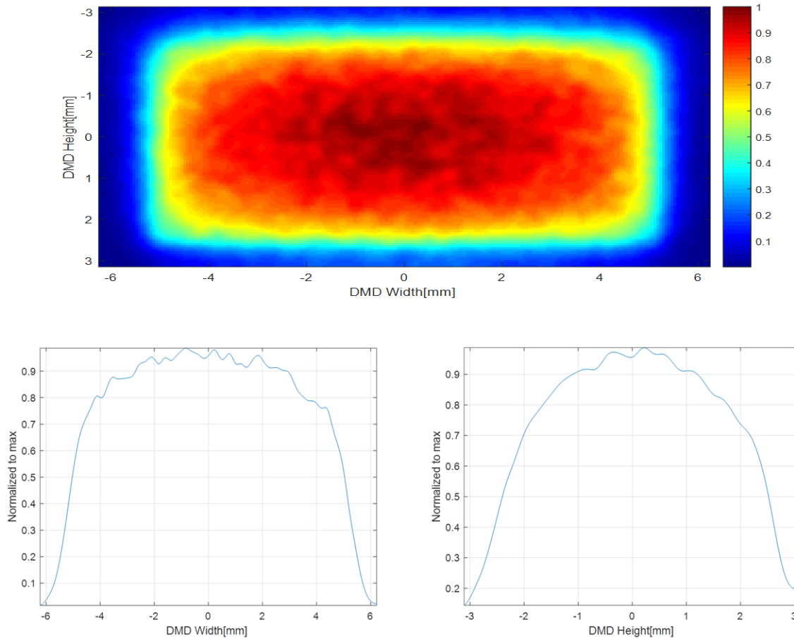
图 7-5. Non-Uniform Illumination Profile
