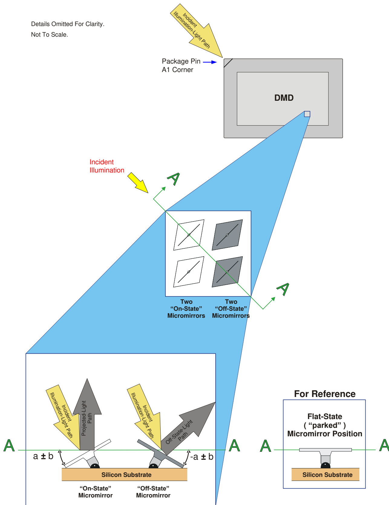
图 7-3. Micromirror States: On, Off, Flat
